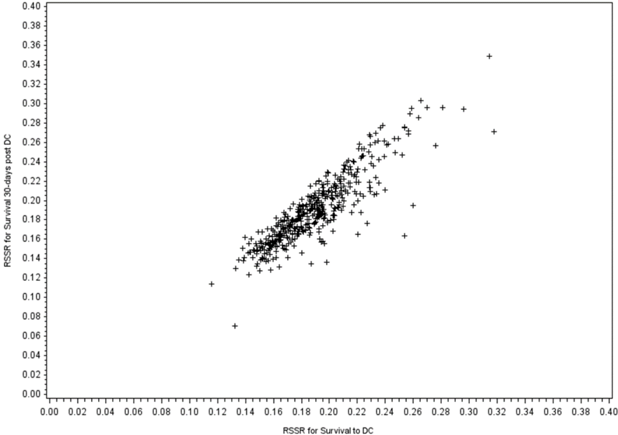
Figure 1. Correlation of a Hospital's RSSR for in-hospital survival and 30-day survival for IHCA
