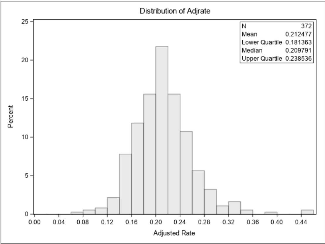
Figure 2. Distribution of Adjusted in-hospital survival rate for IHCA
