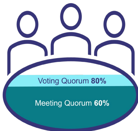
Figure 5. Quorum Thresholds
